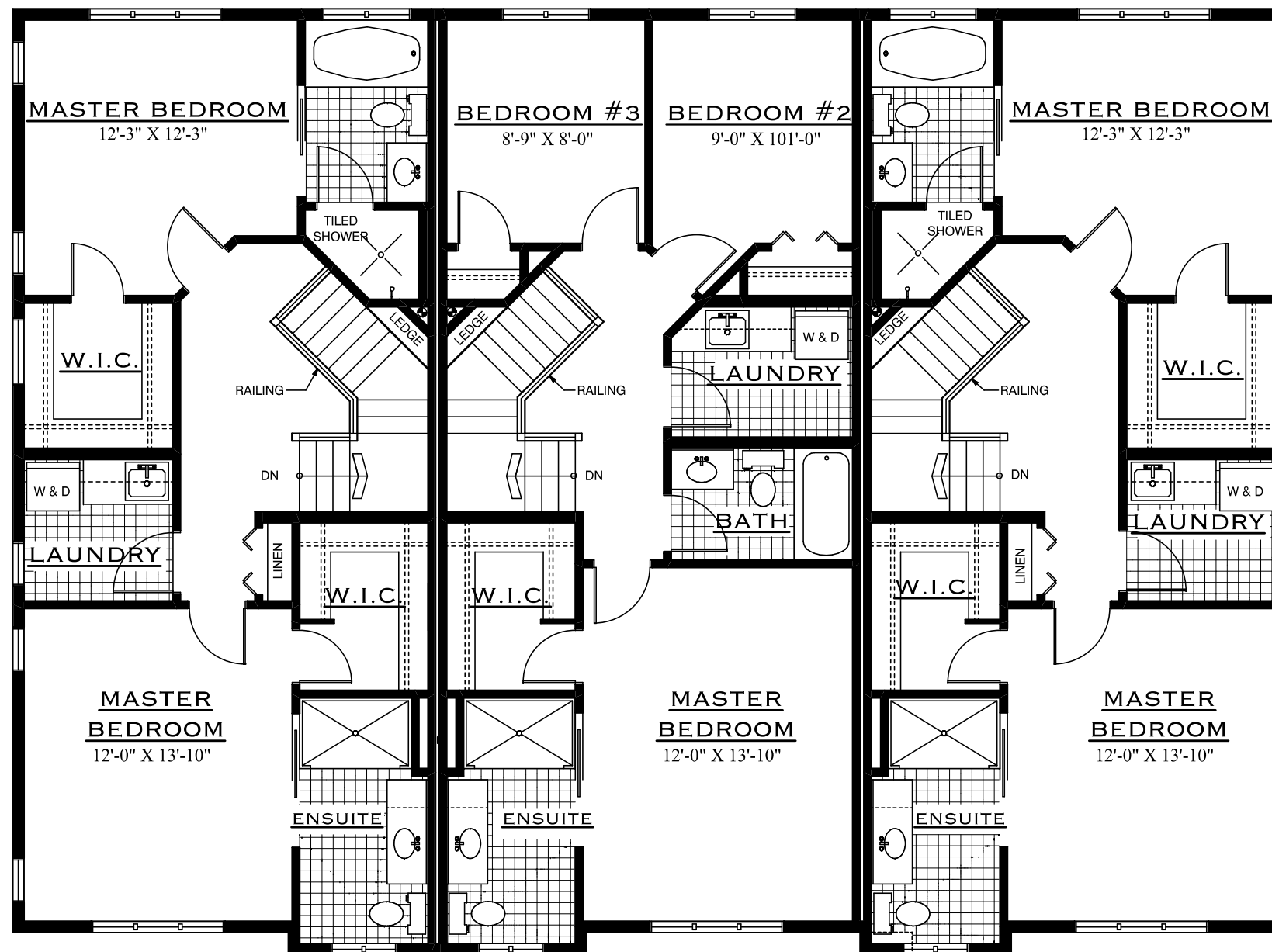
UNIT 1 741 SQ.FT.
